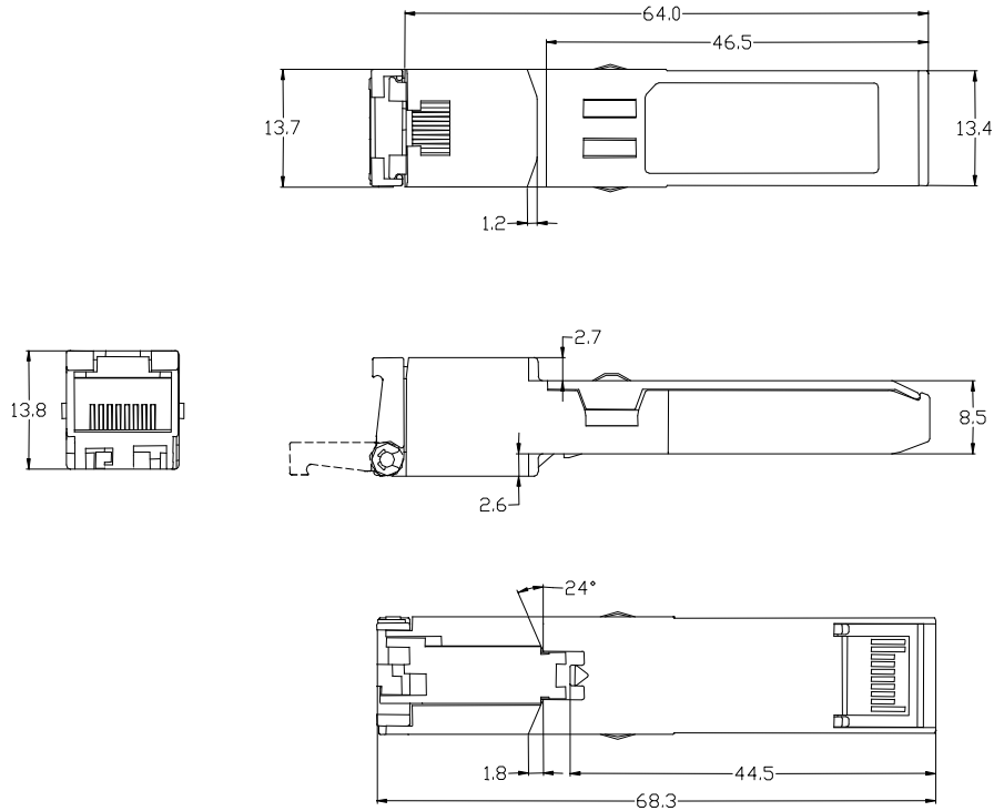
Figure 2. Mechanical Dimensions of Transceiver
