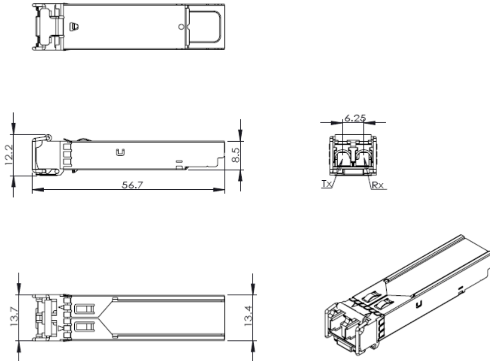
Figure 6. Mechanical Drawing
