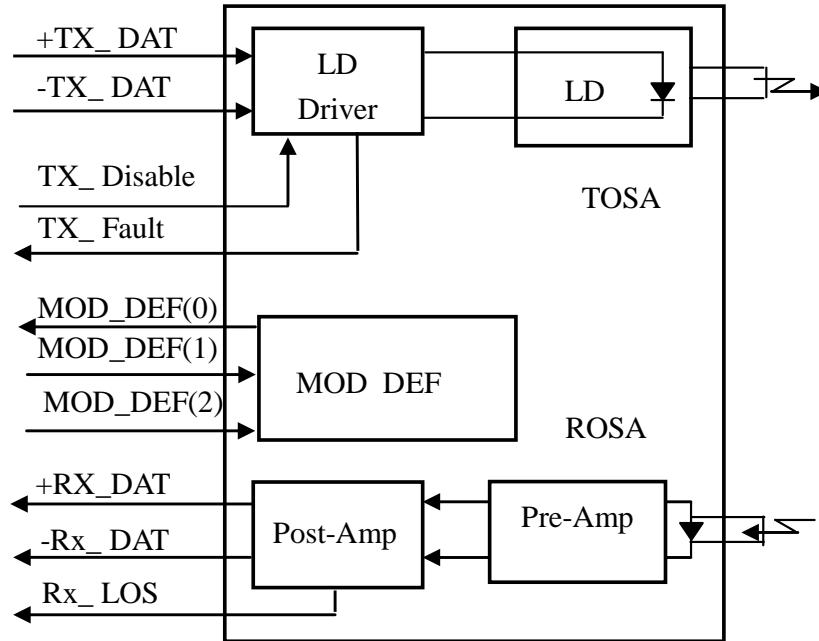
Figure1: Block Diagram
