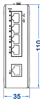
IES2105-4P1T-P48
