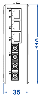
IES2105-3T2F-P48、 IES2105-3T2F-P220
