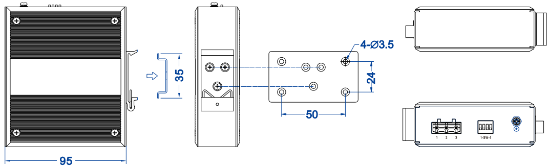
IES2105-4T1F-P48、 IES2105-4T1F-P220
