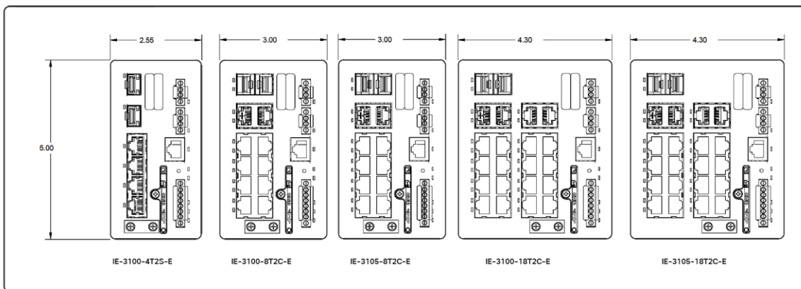
Figure 4. Cisco Catalyst IE3100 front view dimensions
